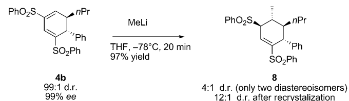
Scheme 3. Addition of MeLi to 4b for the creation of four contiguous stereogenic centers. THF = tetrahydrofuran.
